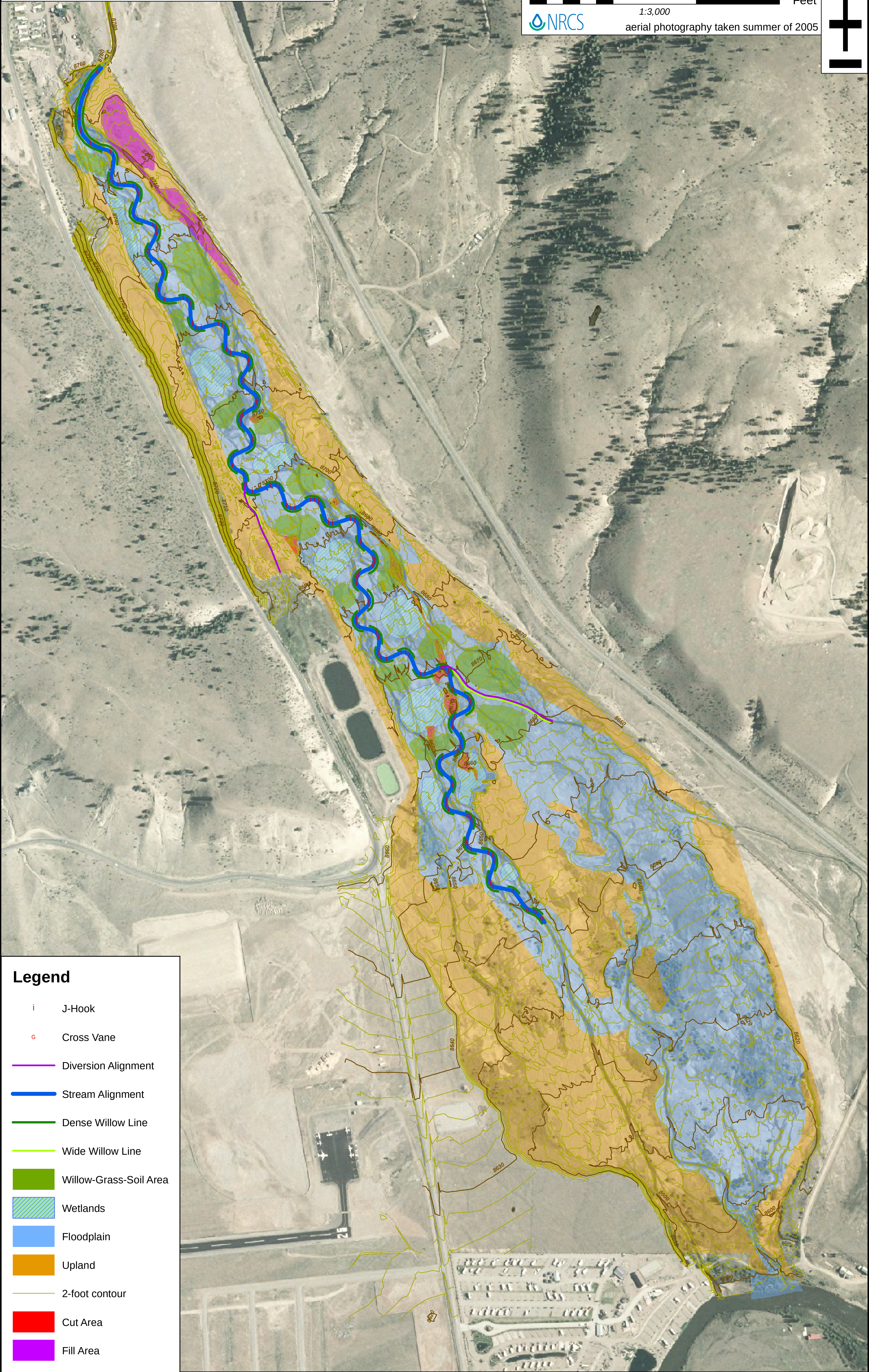
Figure A-11: Restoration Layout, Alternative 3
