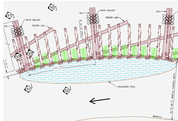
Figure 64: Two cells of a toe wood plan view. This configuration is intended for high-bank locations, with rock-ballasted sills embedded in the bank.
