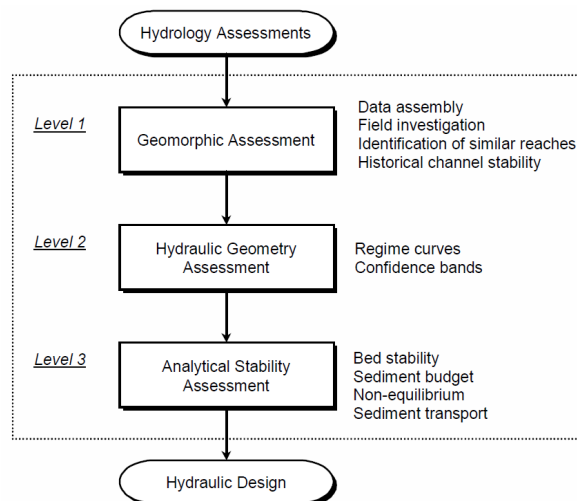
Figure 3: Levels of stability assessments (Copeland et al. 2001).
