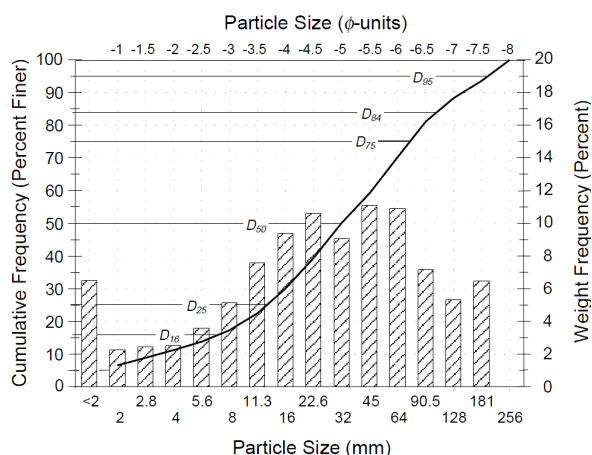
Figure 18: Example bed material particle size distribution (Bunte and Abt 2001).
