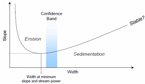
Figure 29: Analytical channel design using the Copeland method (Soar and Thorne 2001).
