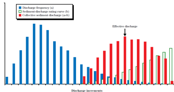
Figure 30: Effective discharge computation (NRCS 2007, Ch5).
