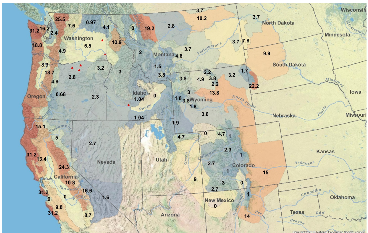
Figure 24: Flood potential zones and index values for a portion of the Western United States. The warmer colors and higher values indicate larger historic (and expected) flood magnitudes.
