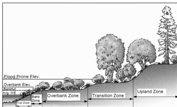
Figure 14: Vegetation zones within a riparian cross section (Hoag et al. 2008).
