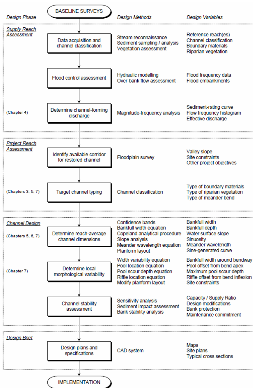
Figure 28: Soar and Thorne (2001) stream restoration design procedure.
