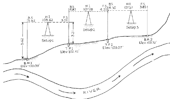
Figure 15: Differential surveying (Harrelson et al. 1994).
