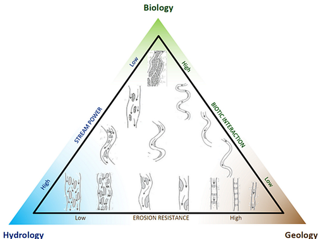
Figure 11: The Stream Evolution Triangle (SET) with planform patterns defined by Schumm (1985) illustrating typical planforms expected to occur in different process-domains. The SET represents the relative influences of geology (erosion resistance), hydrology (stream power), and biology (biotic interaction). From Castro and Thorne (2019).
