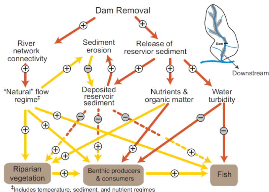
Figure 74: Causal loop diagram illustrating mechanistic links and feedback loops for locations downstream of a dam removal (Bellmore et al., 2019).
