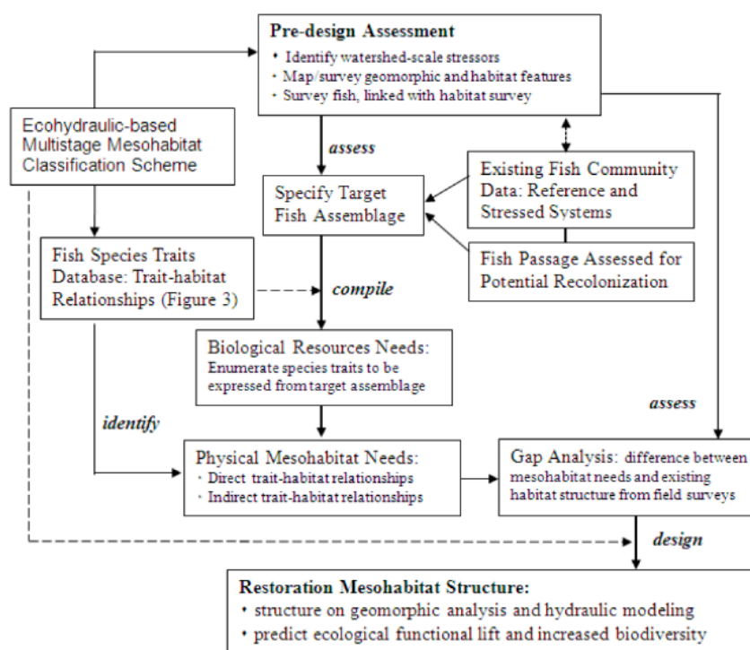
Figure 45: Proposed restoration design strategy utilizing ecohydraulic principles and species functional traits (Schwartz 2016).
