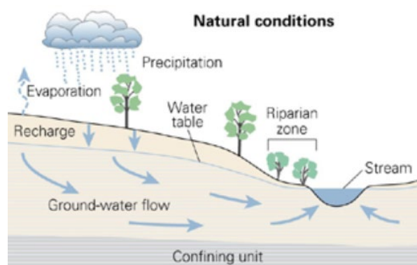
Figure 34: Schematic illustrating a valley cross section for a gaining stream reach (USDA Forest Service, 2007)
