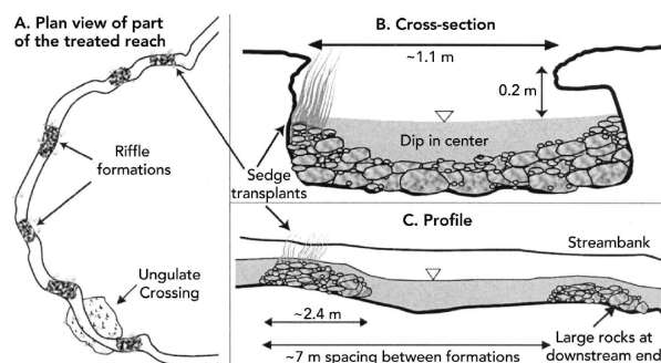
Figure 71: Bed stabilization in a wet meadow using constructed riffles (Medina and Long 2004).
