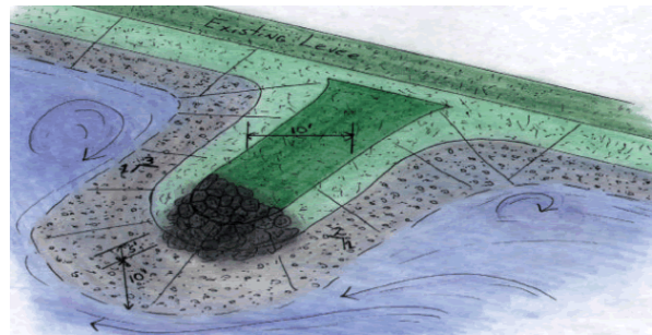
Figure 60: Spur dike (Walla Walla District USACE via Google Images).
