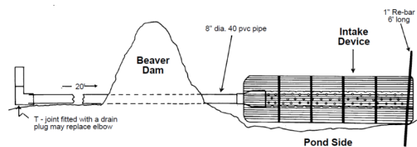
Figure 54: Beaver baffle (Clemson University 1994).
