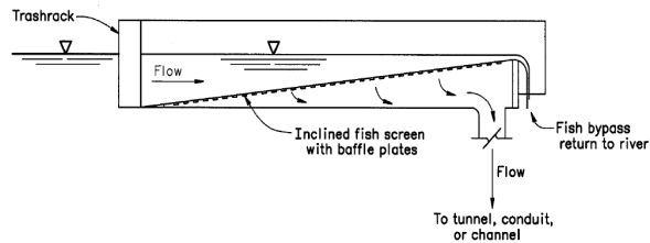
Figure 51: Fixed, inclined fish screen (courtesy Burgi et al. 2006).
