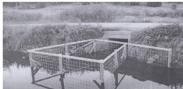
Figure 53: Beaver deceiver (Brown et al. 2001).
