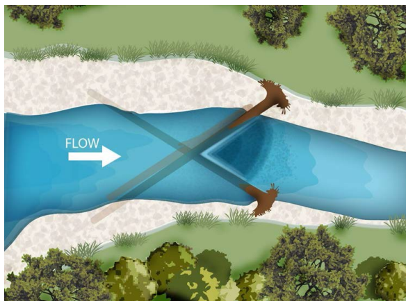
Figure 68: Large wood grade-control structure (Knutson and Fealko 2014).
