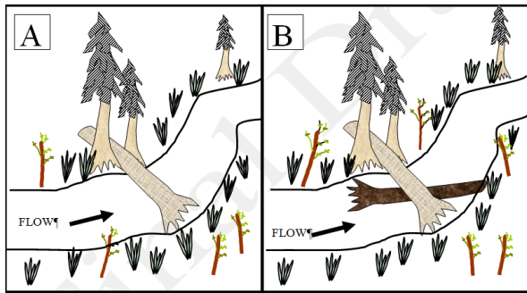
Figure 41: Windthrow emulation, with a single log placed between two standing trees to create a pivot and lock point (A), and with the addition of a second log with rootwad attached to create an X pattern (B). To increase stability, logs should be \geq 1.5 times the bankfull width (with attached rootwad) or \geq 2 times the bankfull width (without an attached rootwad). (Graphic and guidance from ODF ODFW 2010).
