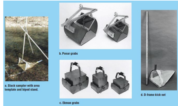
Figure 13: Macroinvertebrate sampling equipment (Moulton et al. 2002).
