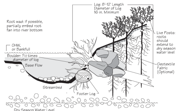
Figure 62: Rootwad with footer section (Eubanks and Meadows 2002).
