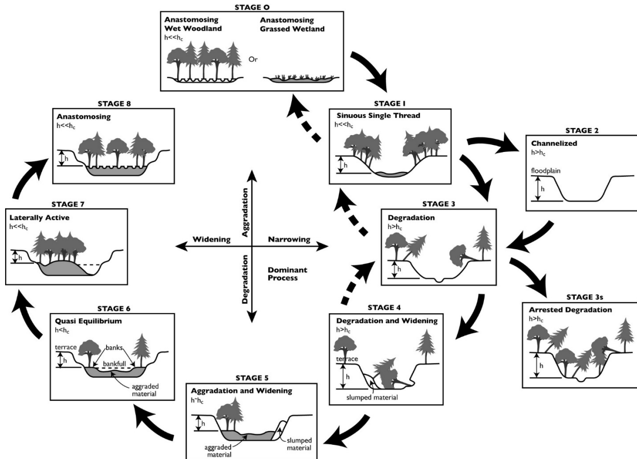
Figure 7: Stream evolution model (Cluer and Thorne 2013). Stage descriptions are provided in Table 5. Dashed arrows indicate "short circuits" in the normal progression.
