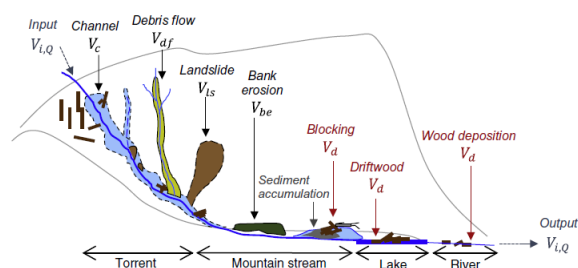
Figure 40: Conceptual visualization of large wood recruitment, transport, and deposition (Steeb et al. 2017).
