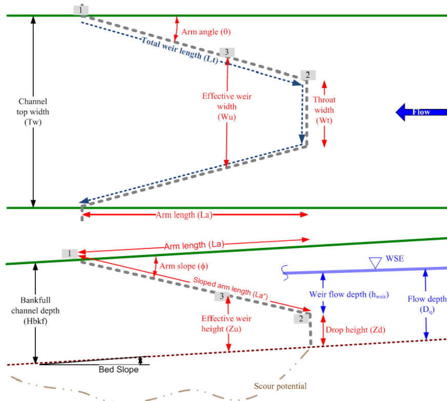
Figure 70: Variable descriptions for U-vane stage-discharge rating (Holmquist-Johnson 2011).
