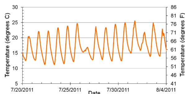
Figure 17: Diurnal temperature fluctuations.
