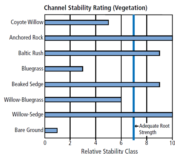
Figure 35: Channel stability ratings for various vegetative compositions (Wyman et al. 2006).
