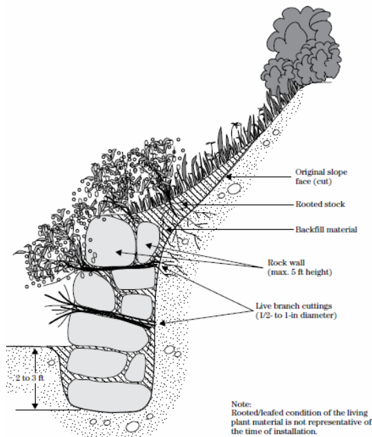
Figure 66: Vegetated rock wall (NRCS 2007, TS-14M).
