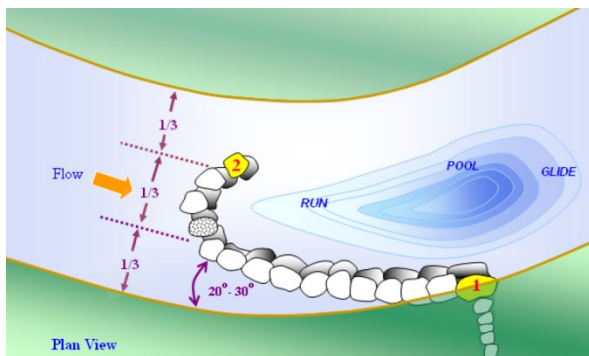
Figure 56: J-hook vane (NRCS 2007).
