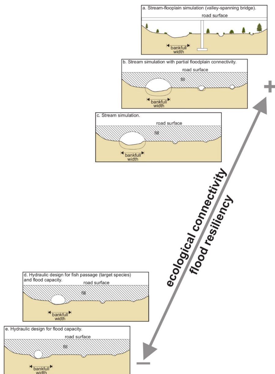
Figure 48: Spectrum of road crossing impacts upon aquatic organism passage and flood resiliency (graphic courtesy of Dan Cenderelli).
