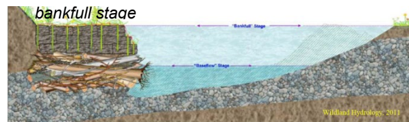
Figure 63: Toe wood cross section (Wildland Hydrology).
