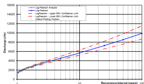
Figure 23: Flow frequency estimates for the Cache la Poudre River, CO (USGS 06752000).
