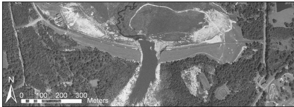
Fig. 1. Big Bay Reservoir embankment
