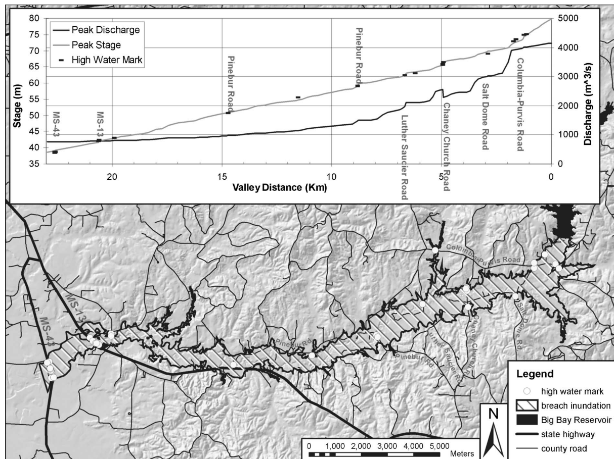
Fig. 2. Big Bay breach flood inundation, plan and profile
